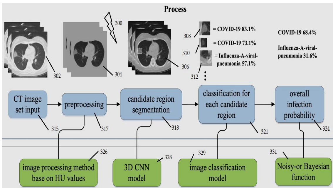
Fig.3: COVID-19 Detection, Spread Prevention and Medical Assistance Using Machine Learning
